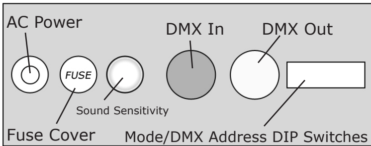
Figure 2: The Rear Connections
