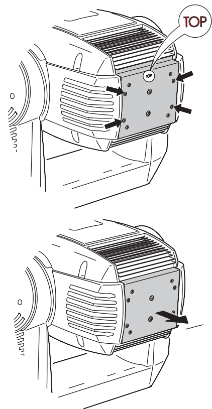
Figure 6: Lamp access
